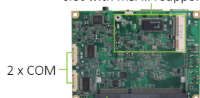
DDR3L SO-DIMM ▲ Rear view
