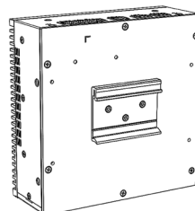
DIN-Rail Assembly
